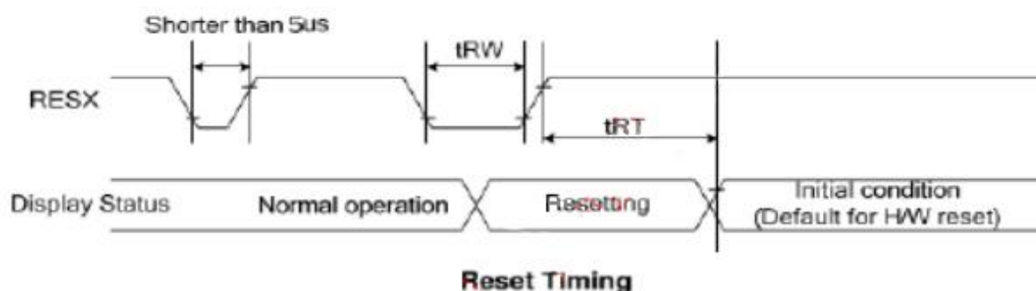
Reset Timing
