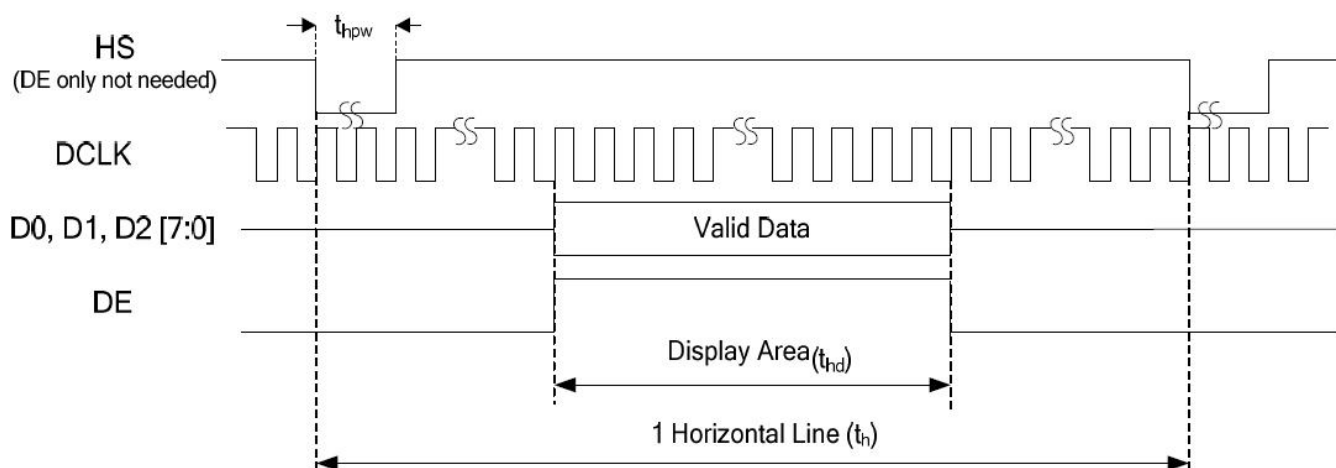
Figure 6-10: Horizontal input timing at DE only mode
