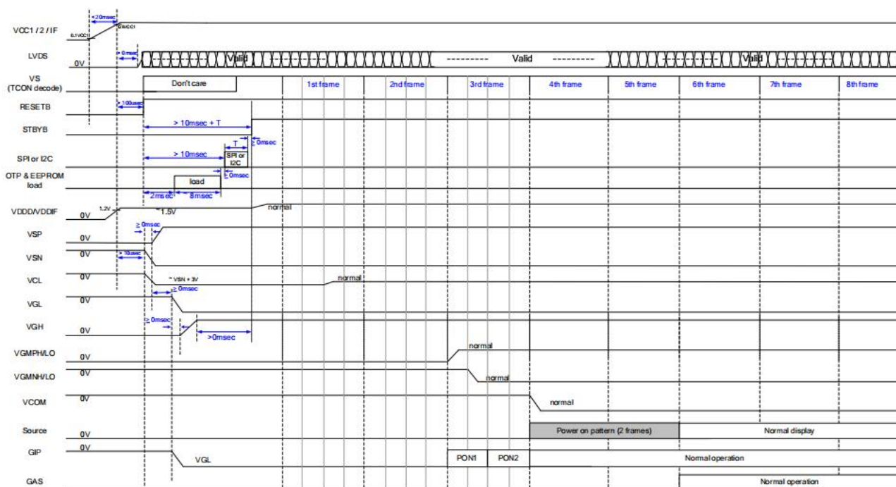
Figure 6-18: Power-on sequence with external VSP/VSN/VGH/VGL (PWR_SPEED=0)
