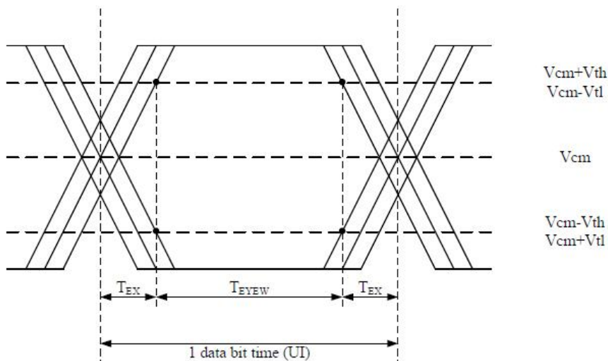
Figure 9-2: LVDS input timing
