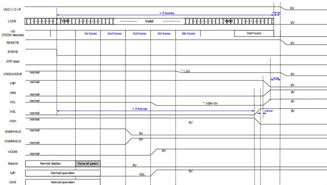
Figure 6-21: Power-off sequence with external VSP/VSN/VGH/VGL
