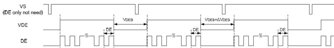
Figure 6-12: Vertical variation timing at DE only mode
