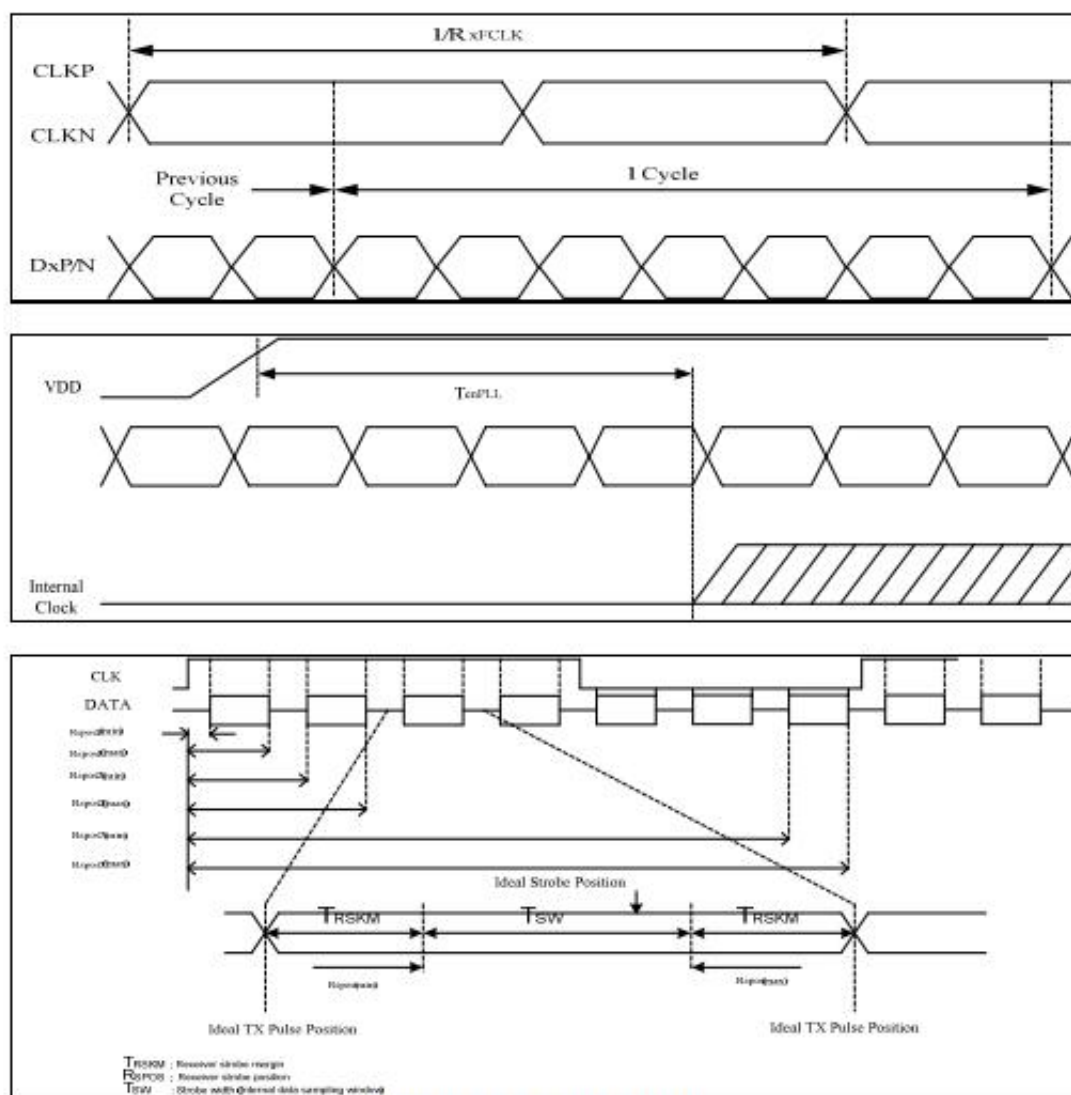
Figure 13.3: LVDS figure
