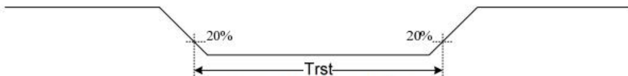
Figure 13.5: Reset timing
