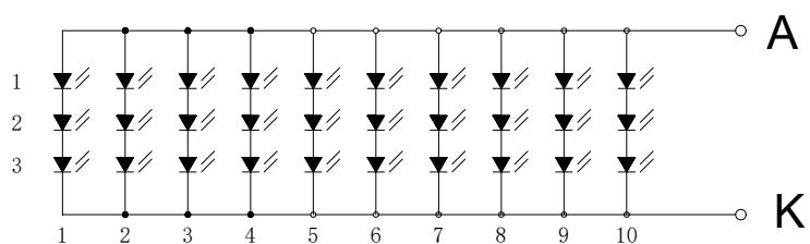
CIRCUIT DIAGRAM
