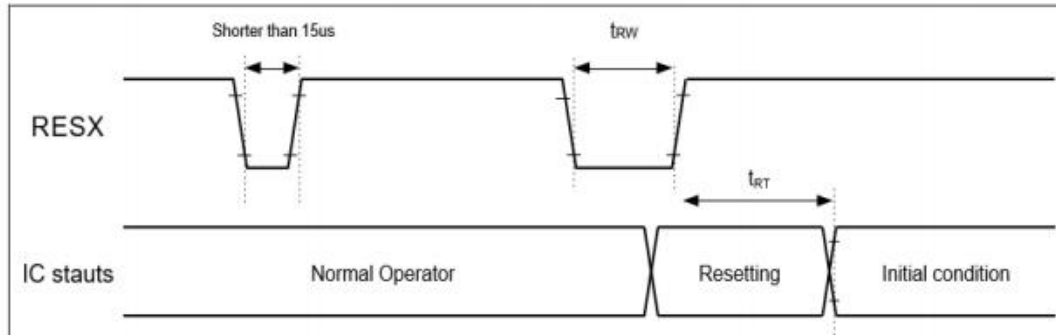
Figure 10.2: Reset input timings
