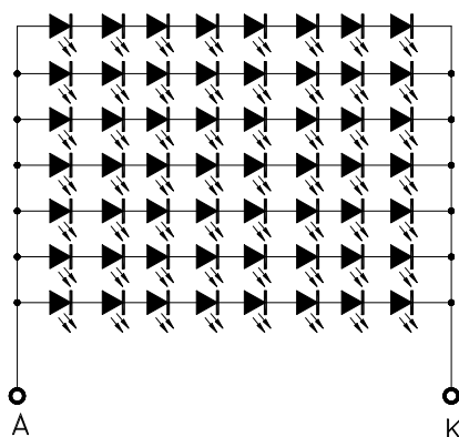
Backlight LED Circuit
