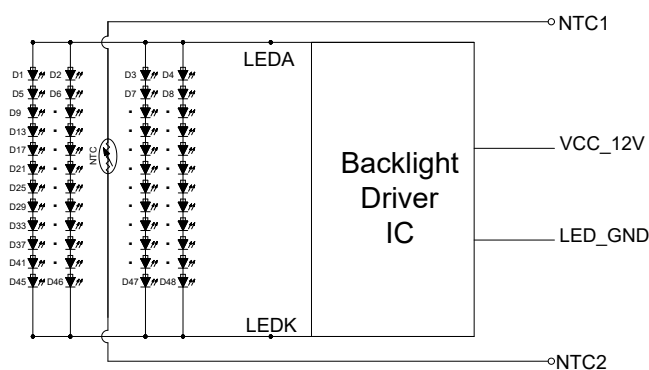
CIRCUIT DIAGRAM VF =32.4~39.6V; IF=170mA
