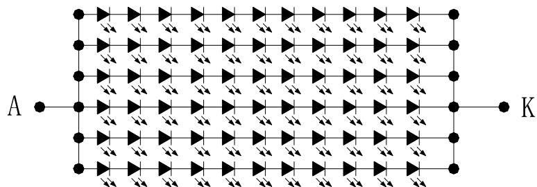
CIRCUIT DIAGRAM
