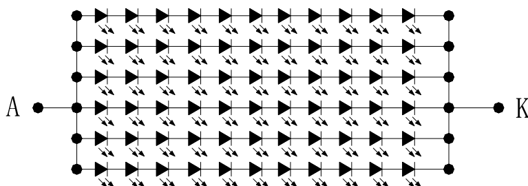
CIRCUIT DIAGRAM
